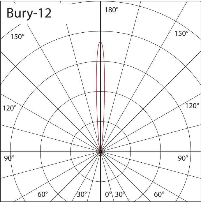
2380Lm at 24W 3000K, 24VDC, CRI>80
