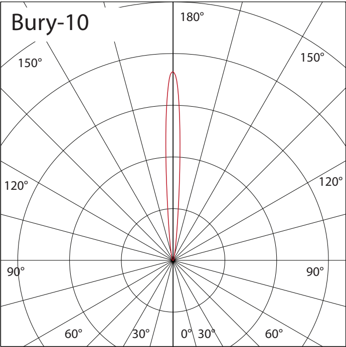
970Lm at 30W 3000K, 24VDC, CRI>80
