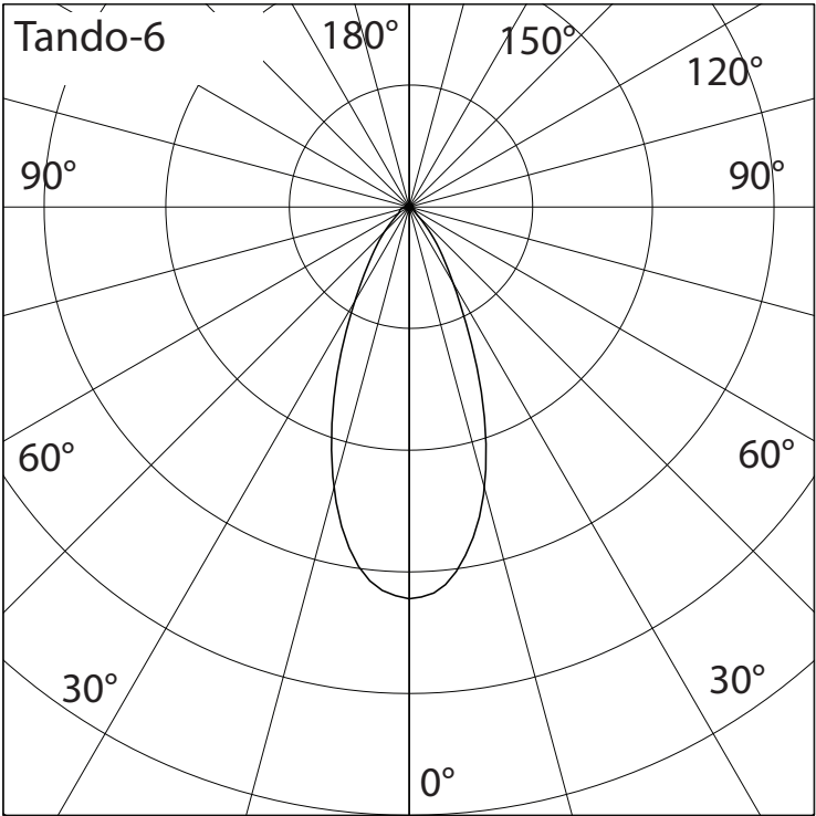
1190Lm At 3000K, 30Deg
