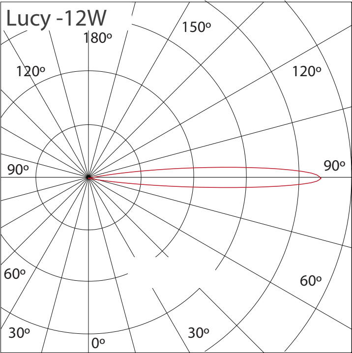
1190Lm At 3000K, 24deg -24VDC
