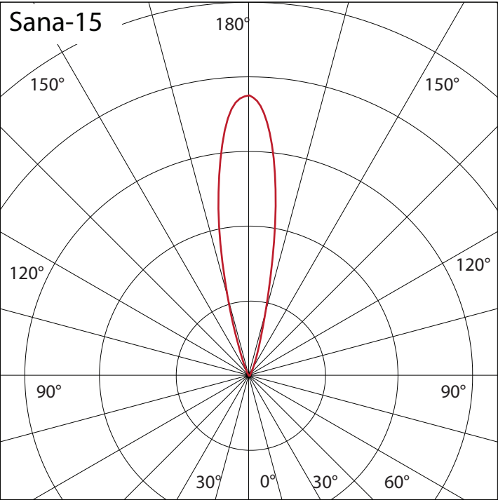
1580Lm at 3000K, 12°
